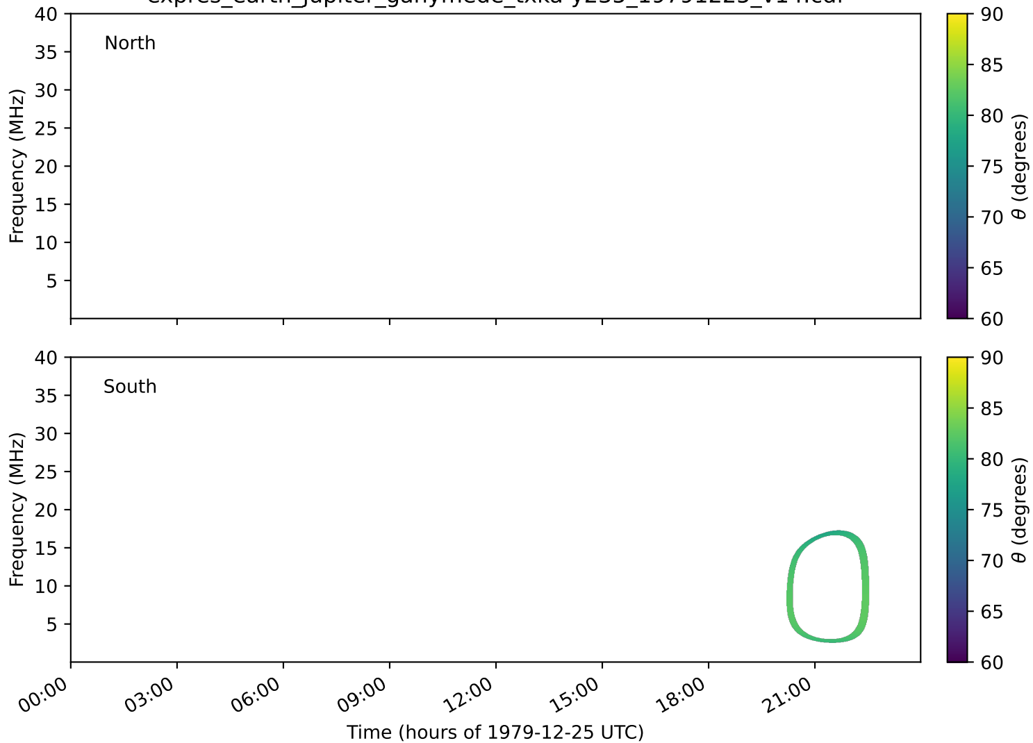
expres_earth_jupiter_ganymede_txka-y235_19791225_v14.cdf
