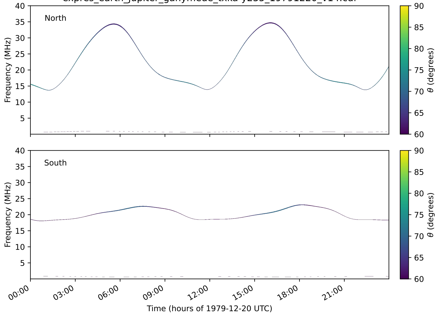
expres_earth_jupiter_ganymede_txka-y235_19791220_v14.cdf
