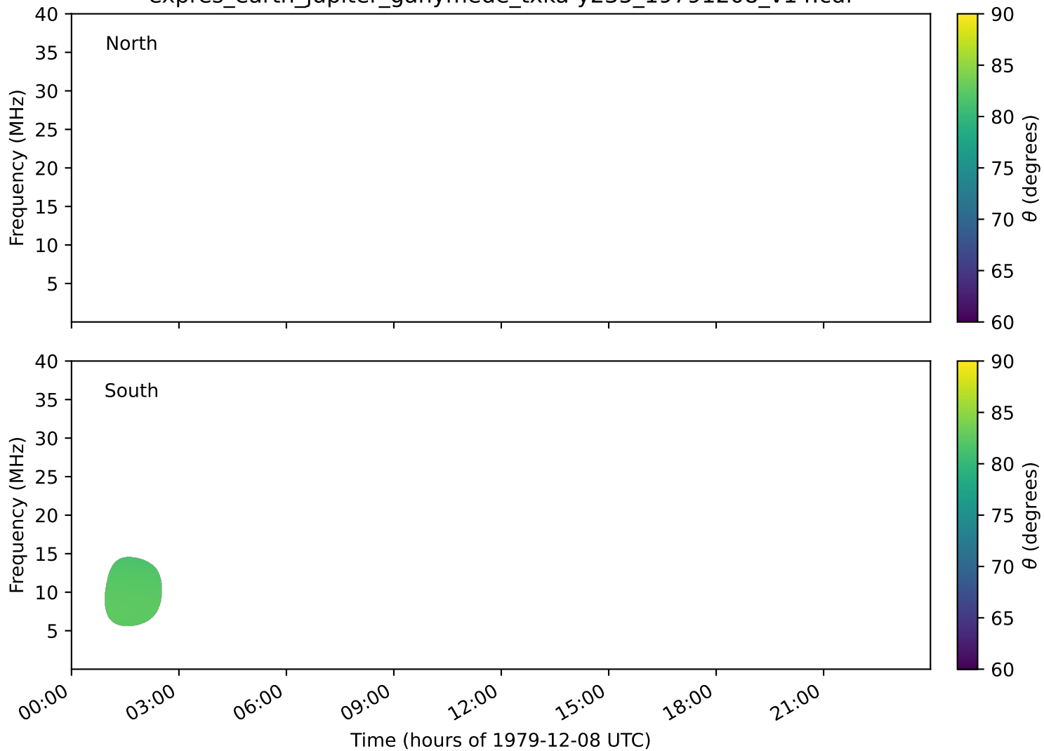
expres_earth_jupiter_ganymede_txka-y235_19791208_v14.cdf
