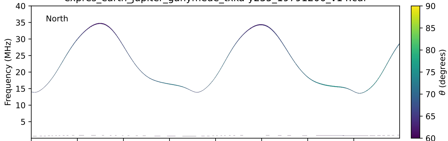
expres_earth_jupiter_ganymede_txka-y235_19791206_v14.cdf
