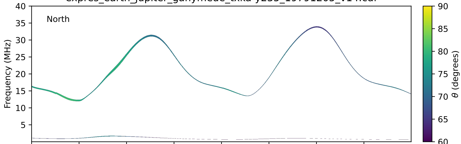
expres_earth_jupiter_ganymede_txka-y235_19791205_v14.cdf
