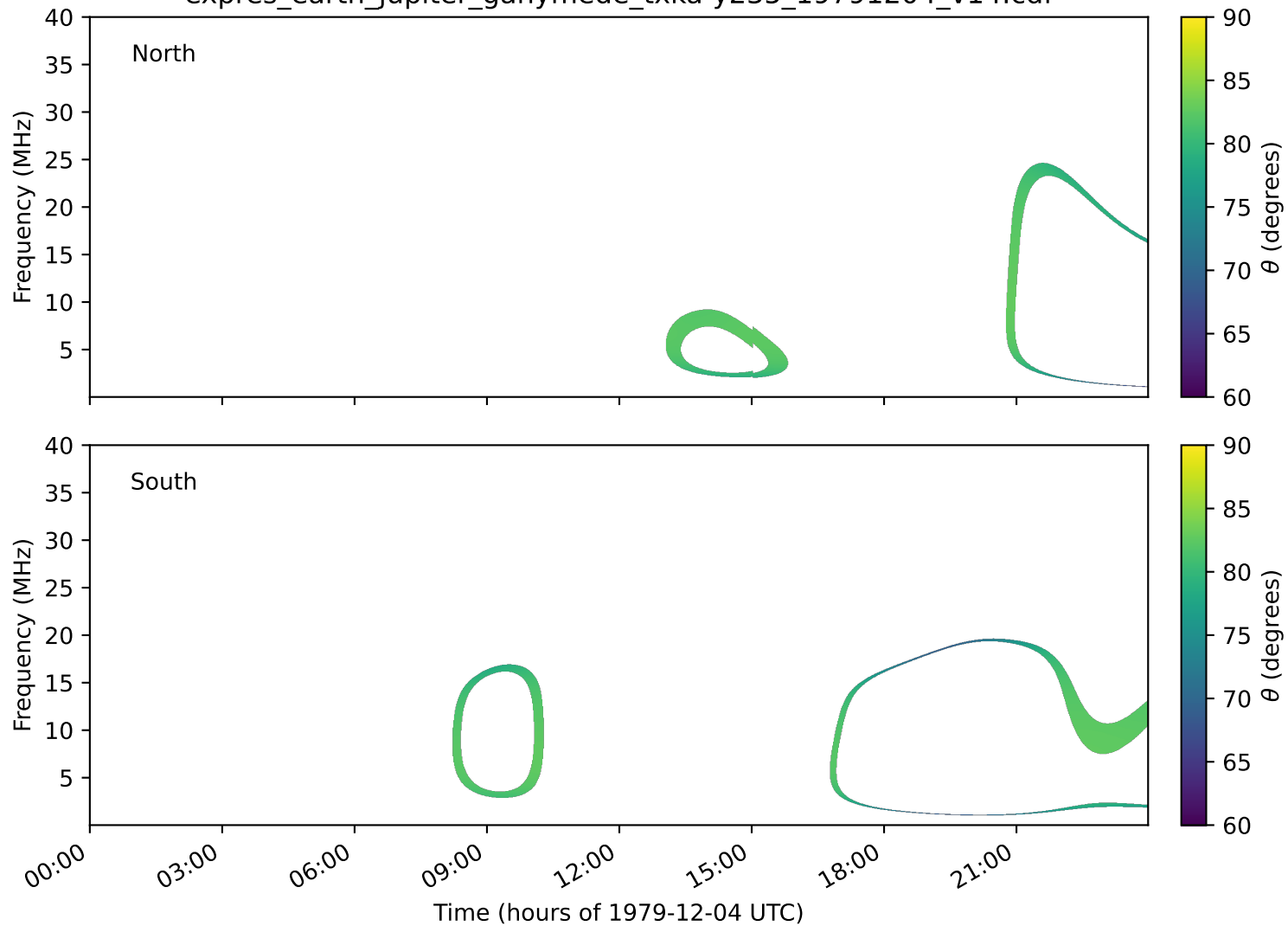
expres_earth_jupiter_ganymede_txka-y235_19791204_v14.cdf
