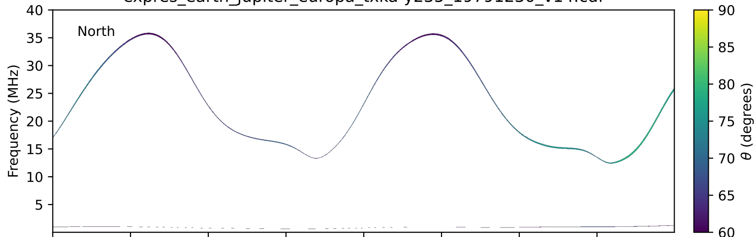
expres_earth_jupiter_europa_txka-y235_19791230_v14.cdf
