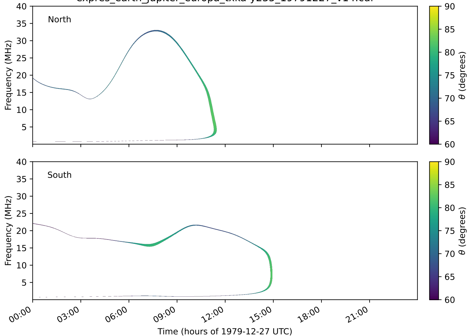
expres_earth_jupiter_europa_txka-y235_19791227_v14.cdf
