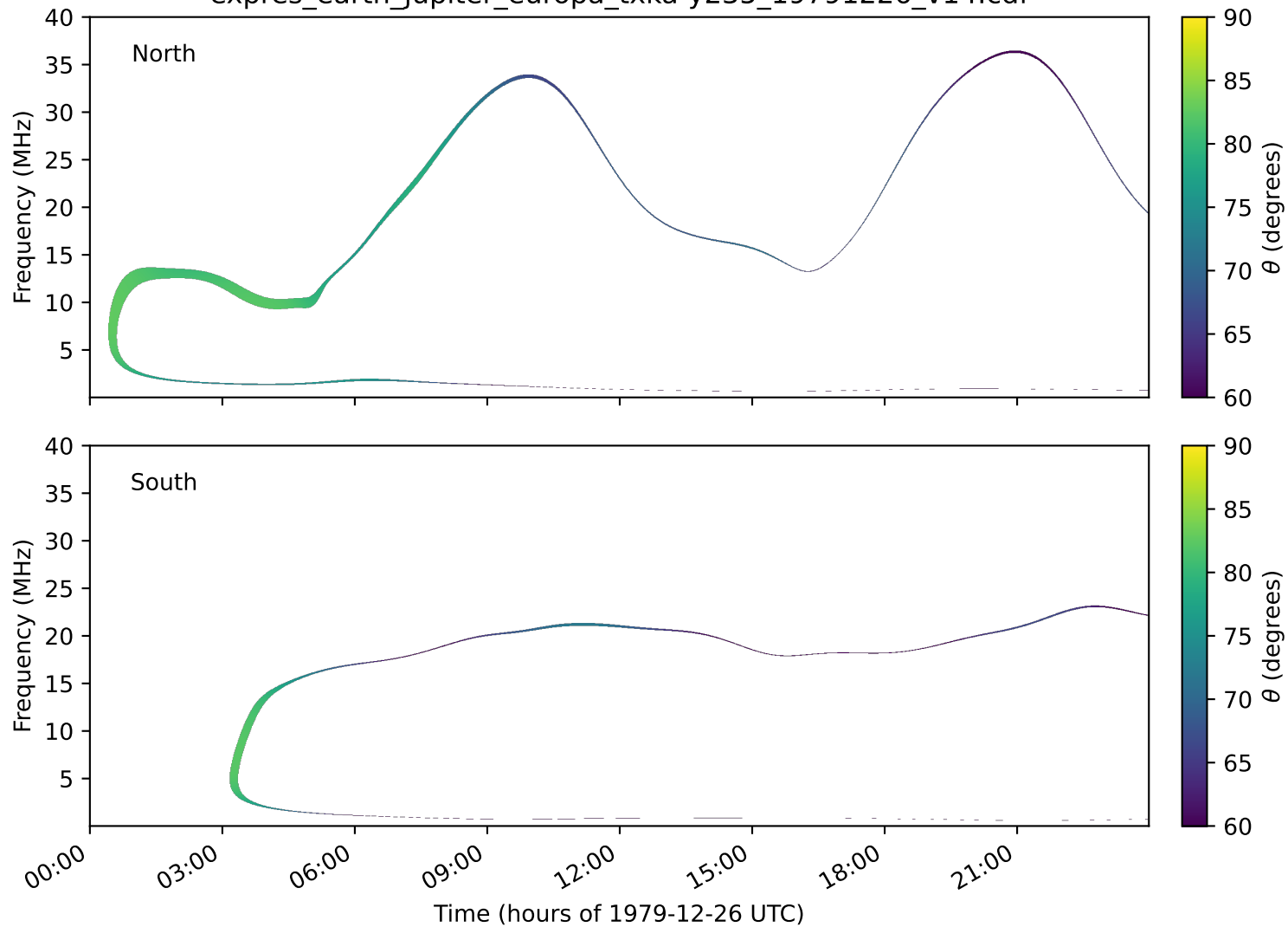
expres_earth_jupiter_europa_txka-y235_19791226_v14.cdf
