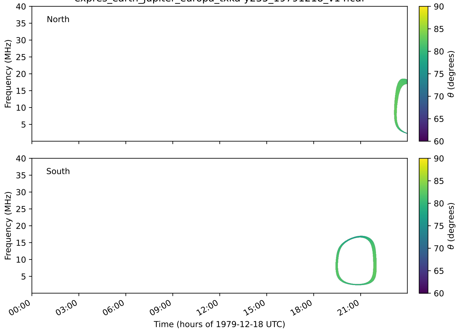
expres_earth_jupiter_europa_txka-y235_19791218_v14.cdf
