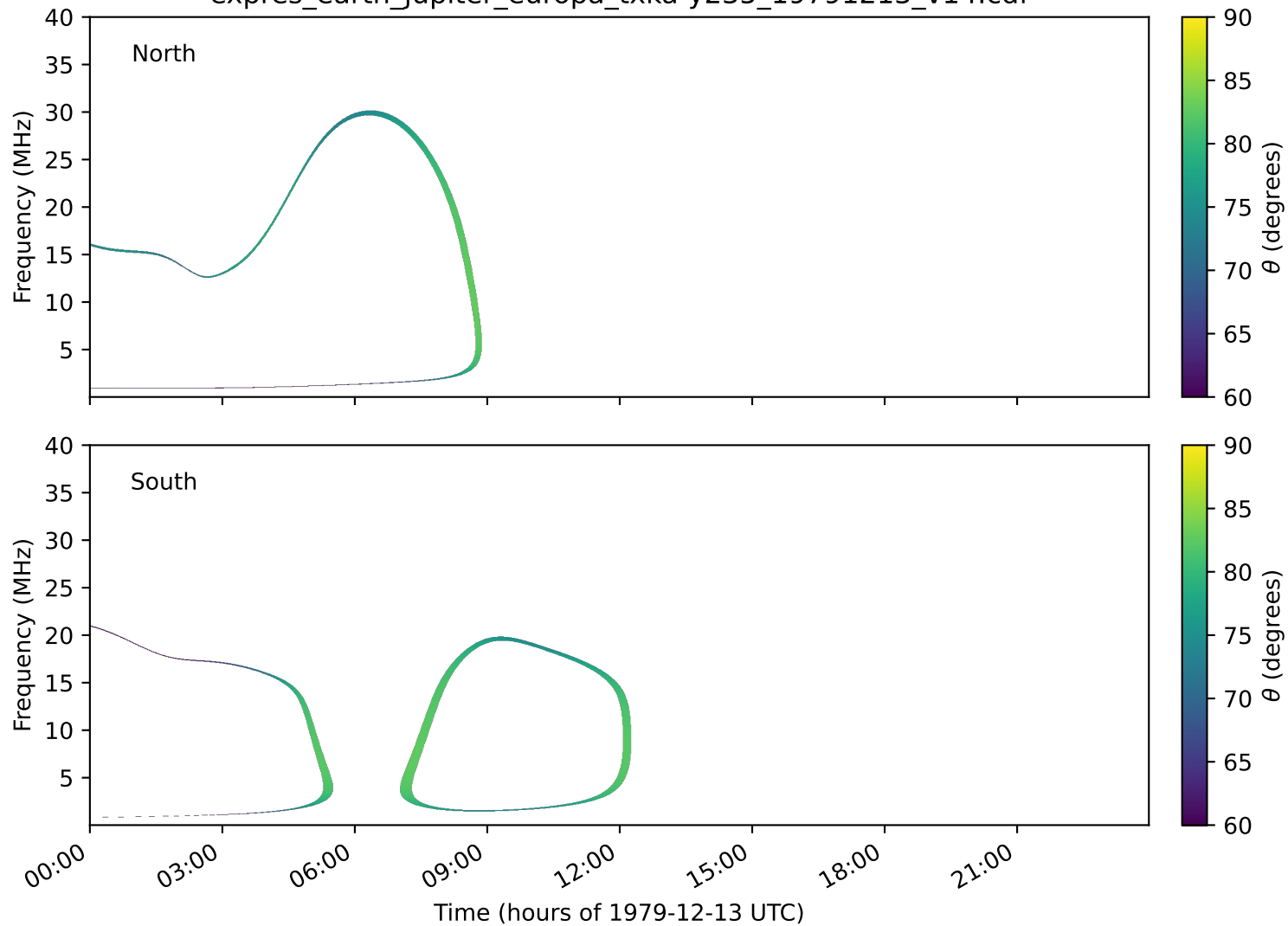
expres_earth_jupiter_europa_txka-y235_19791213_v14.cdf
