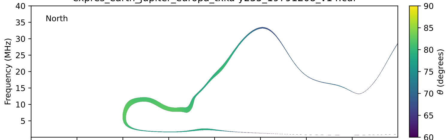
expres_earth_jupiter_europa_txka-y235_19791208_v14.cdf
