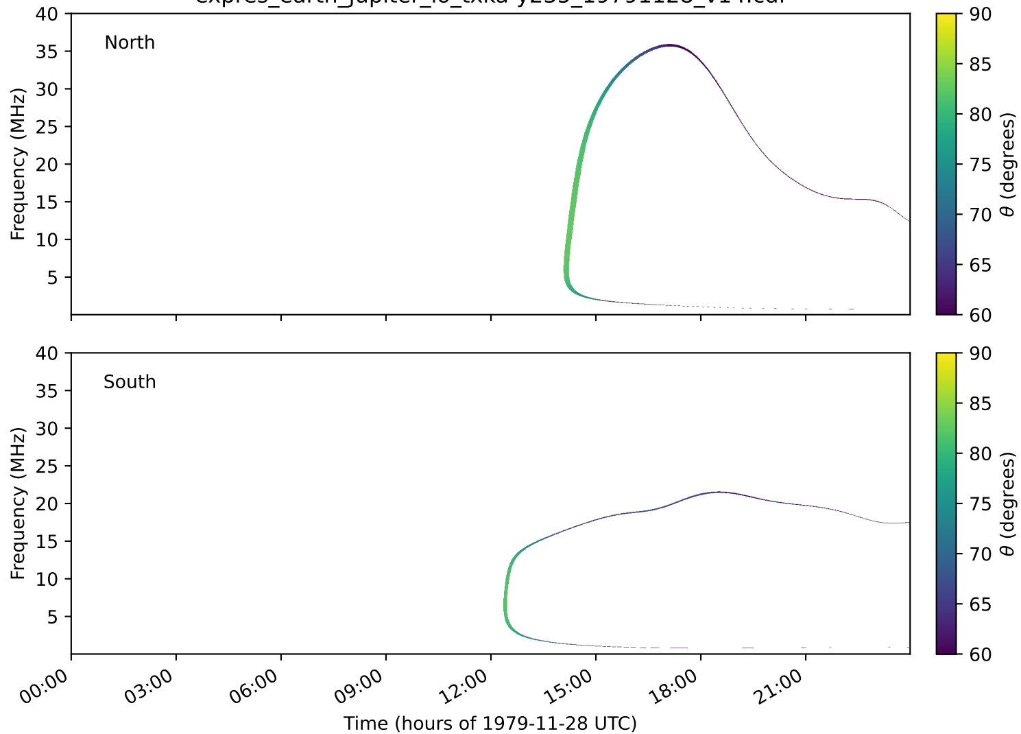
expres_earth_jupiter_io_txka-y235_19791128_v14.cdf
