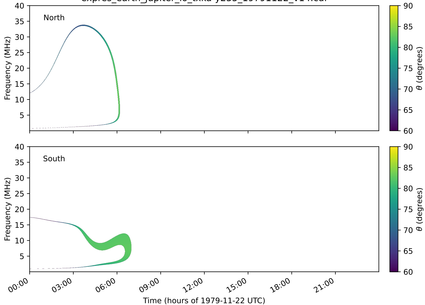
expres_earth_jupiter_io_txka-y235_19791122_v14.cdf
