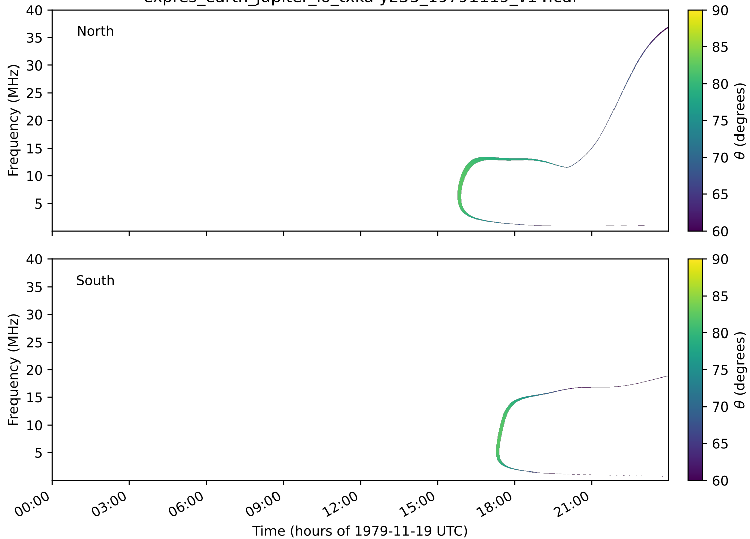
expres_earth_jupiter_io_txka-y235_19791119_v14.cdf
