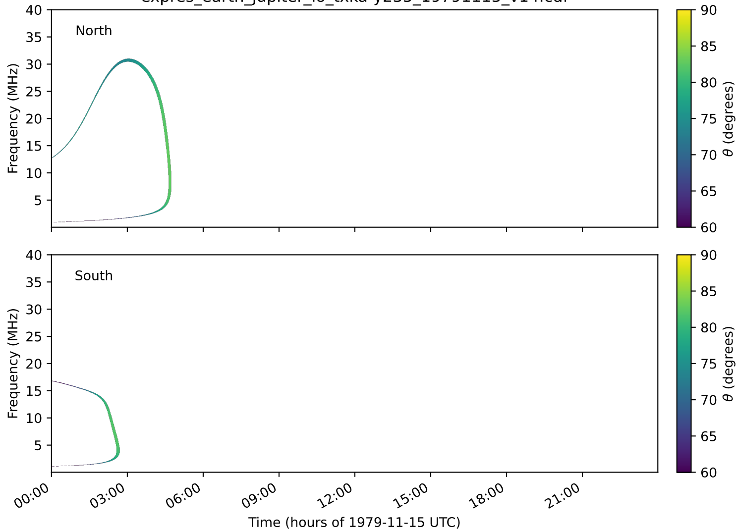
expres_earth_jupiter_io_txka-y235_19791115_v14.cdf
