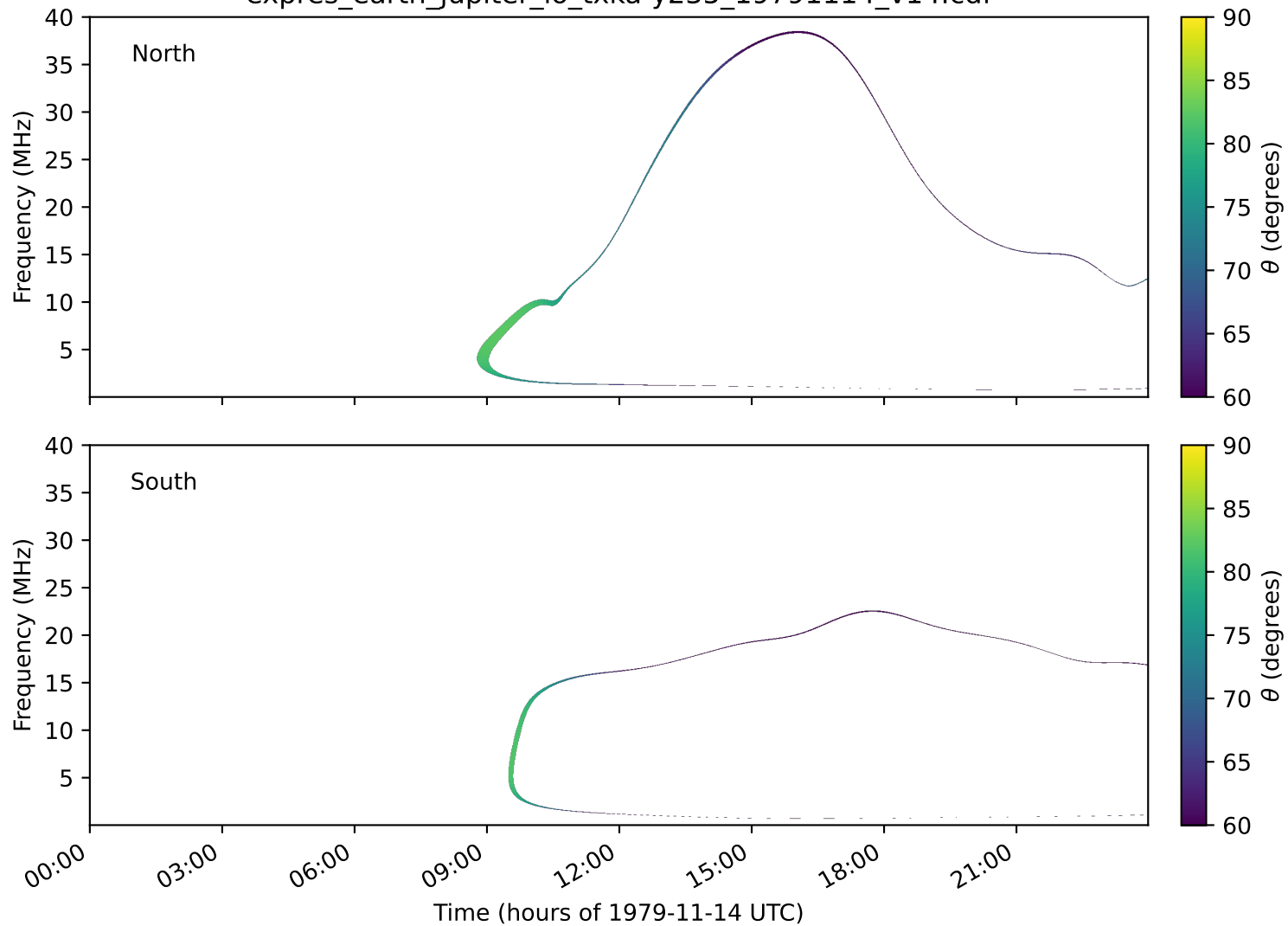
expres_earth_jupiter_io_txka-y235_19791114_v14.cdf
