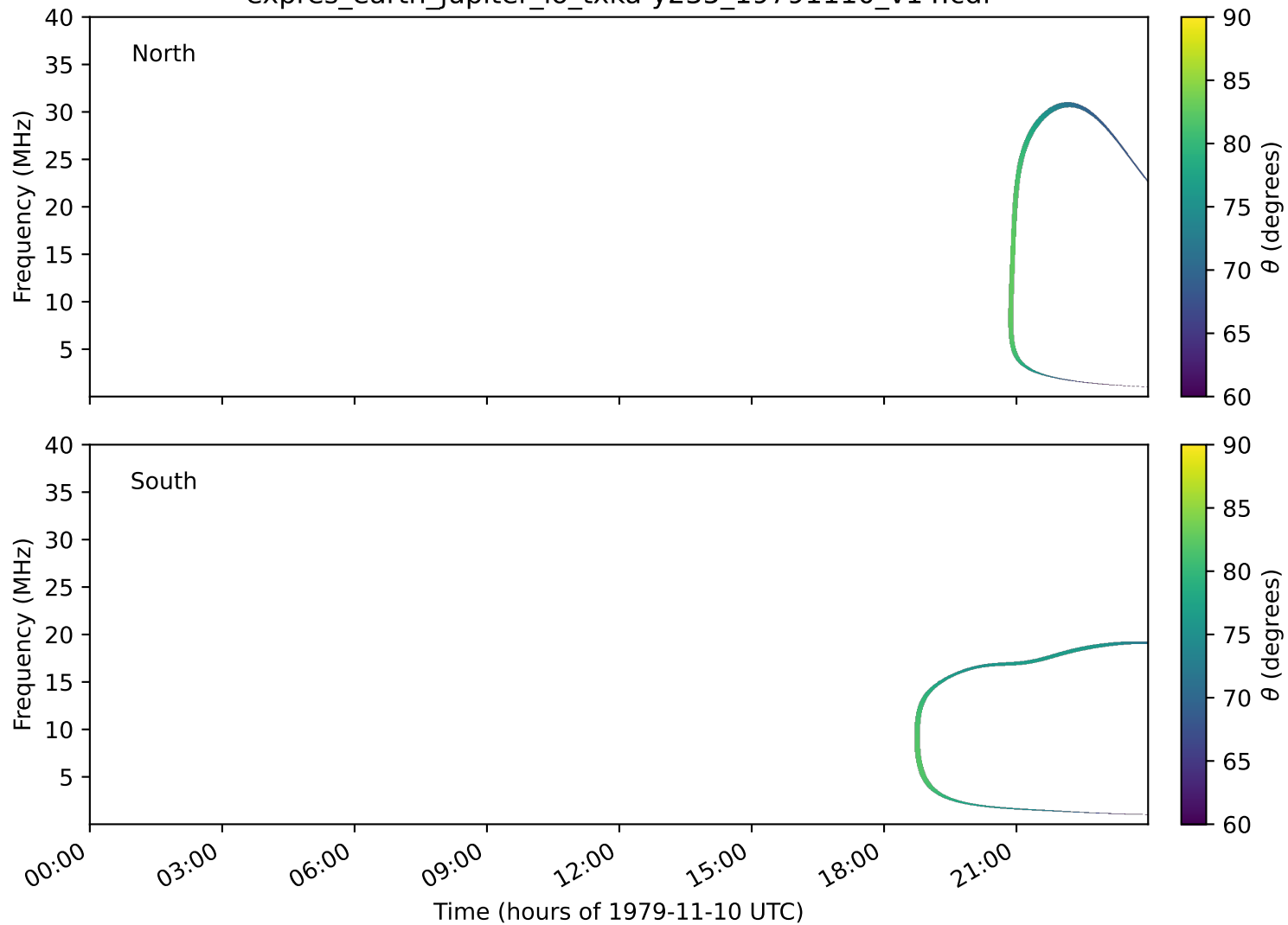
expres_earth_jupiter_io_txka-y235_19791110_v14.cdf
