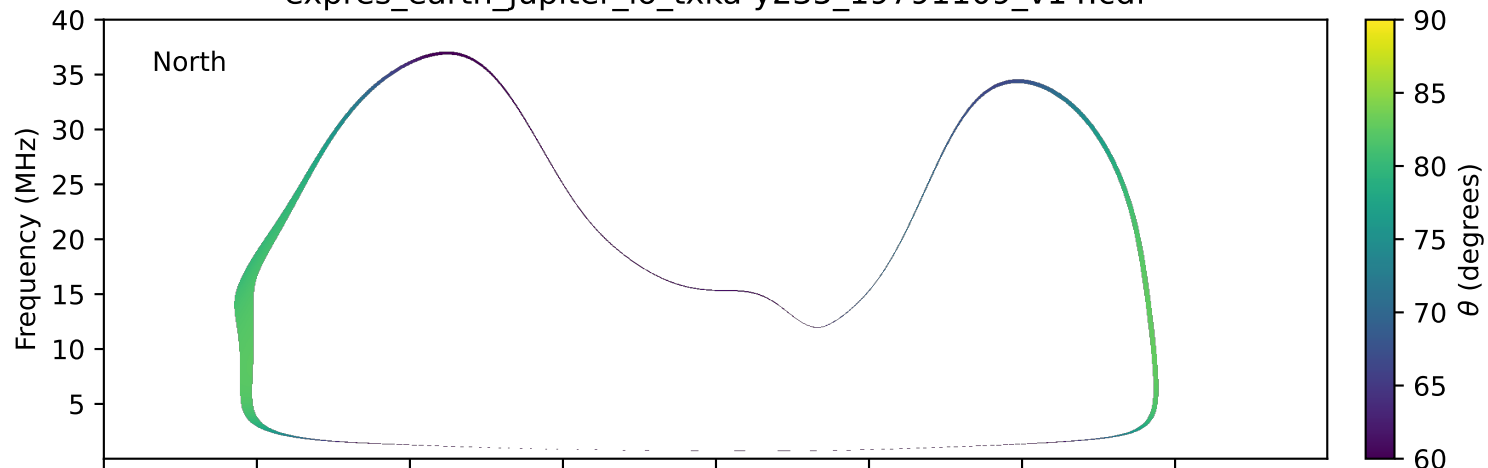
expres_earth_jupiter_io_txka-y235_19791109_v14.cdf
