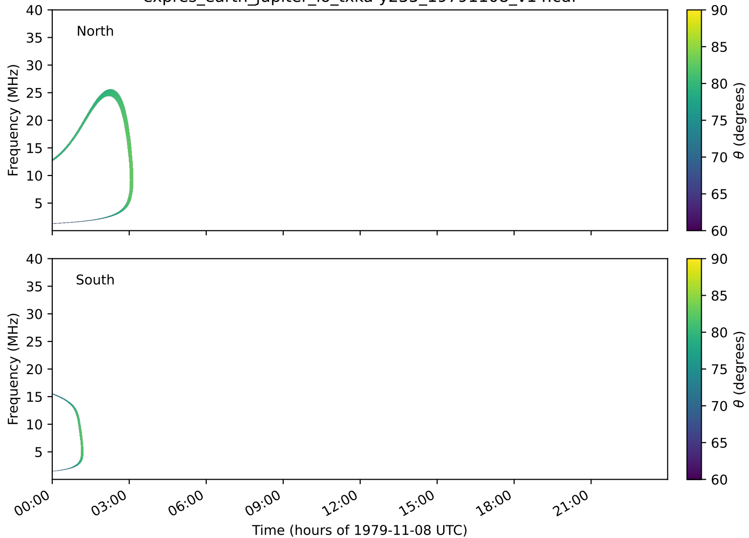
expres_earth_jupiter_io_txka-y235_19791108_v14.cdf
