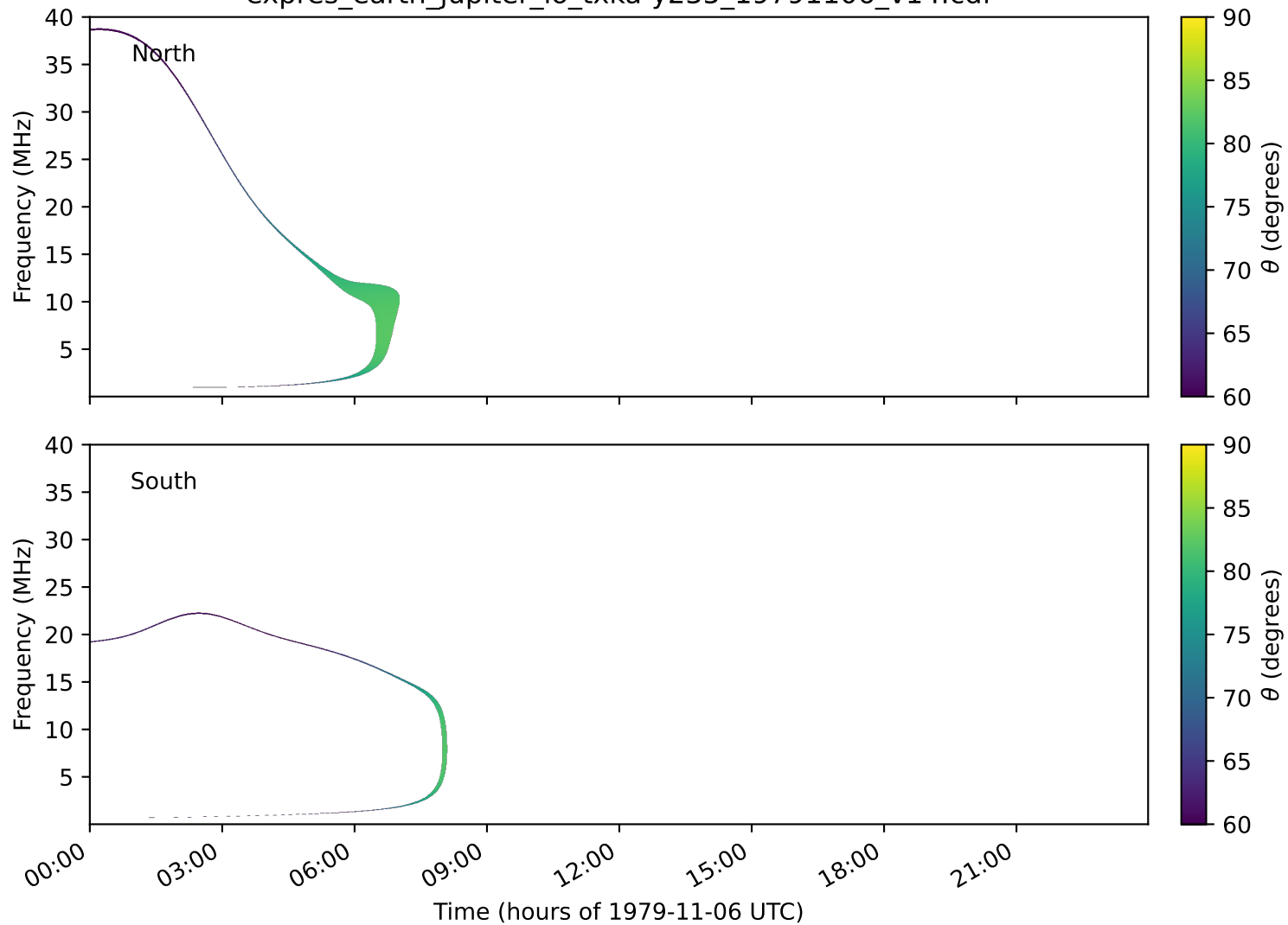
expres_earth_jupiter_io_txka-y235_19791106_v14.cdf
