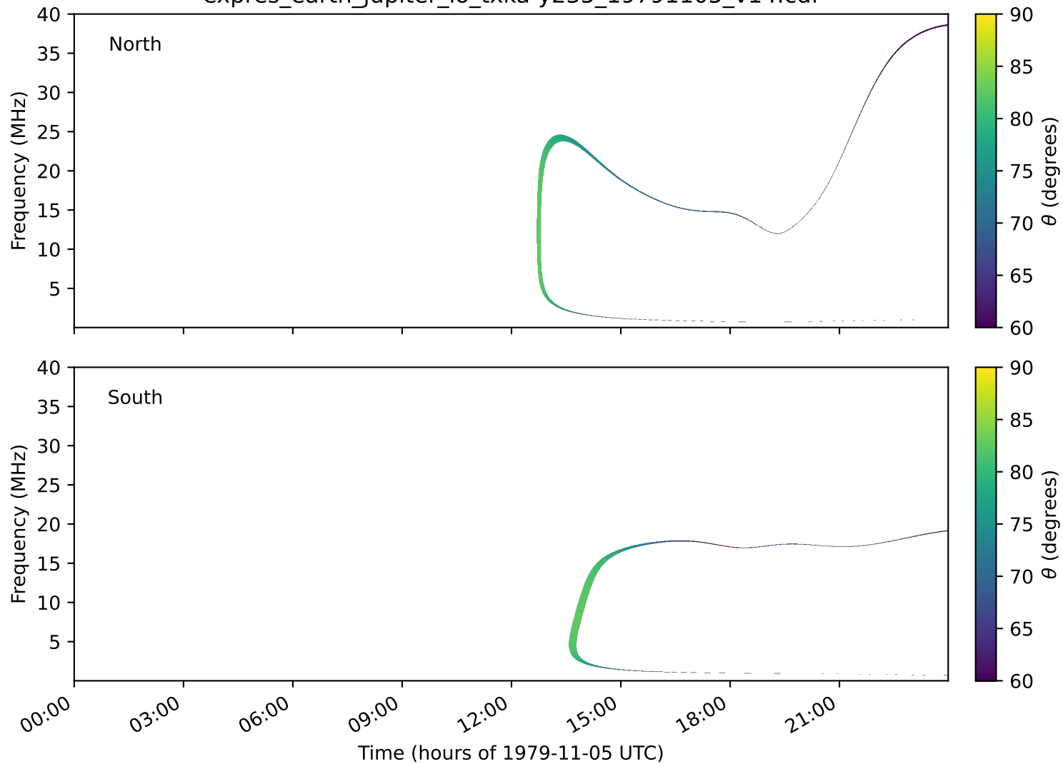
expres_earth_jupiter_io_txka-y235_19791105_v14.cdf
