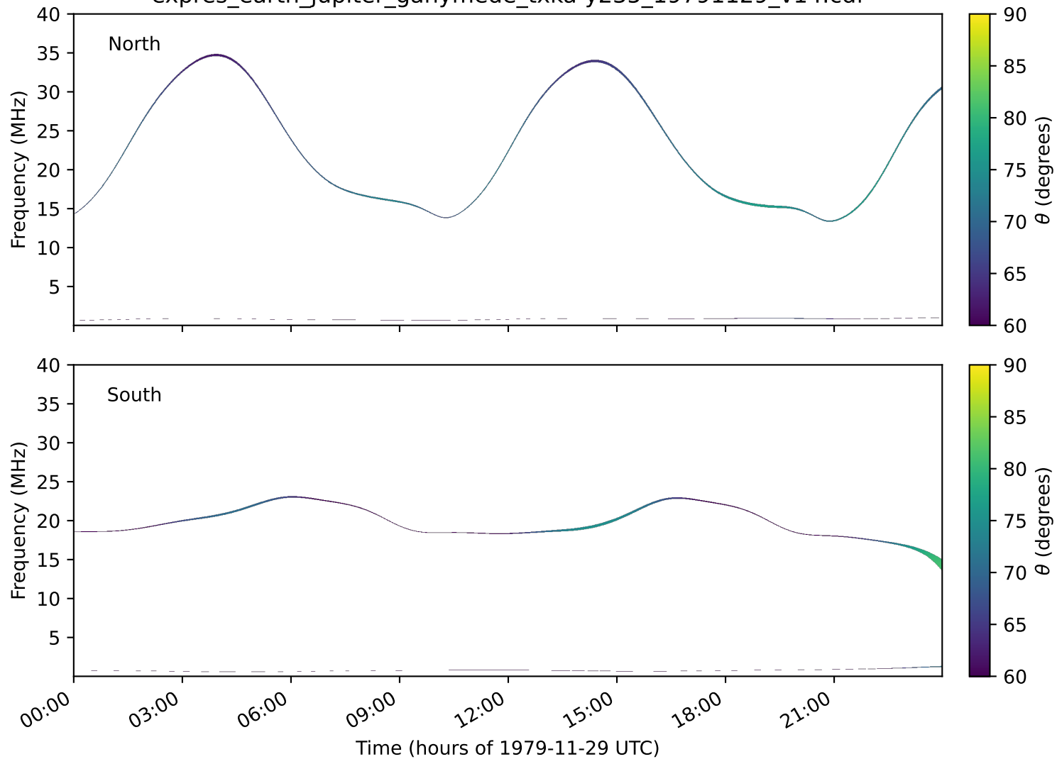
expres_earth_jupiter_ganymede_txka-y235_19791129_v14.cdf
