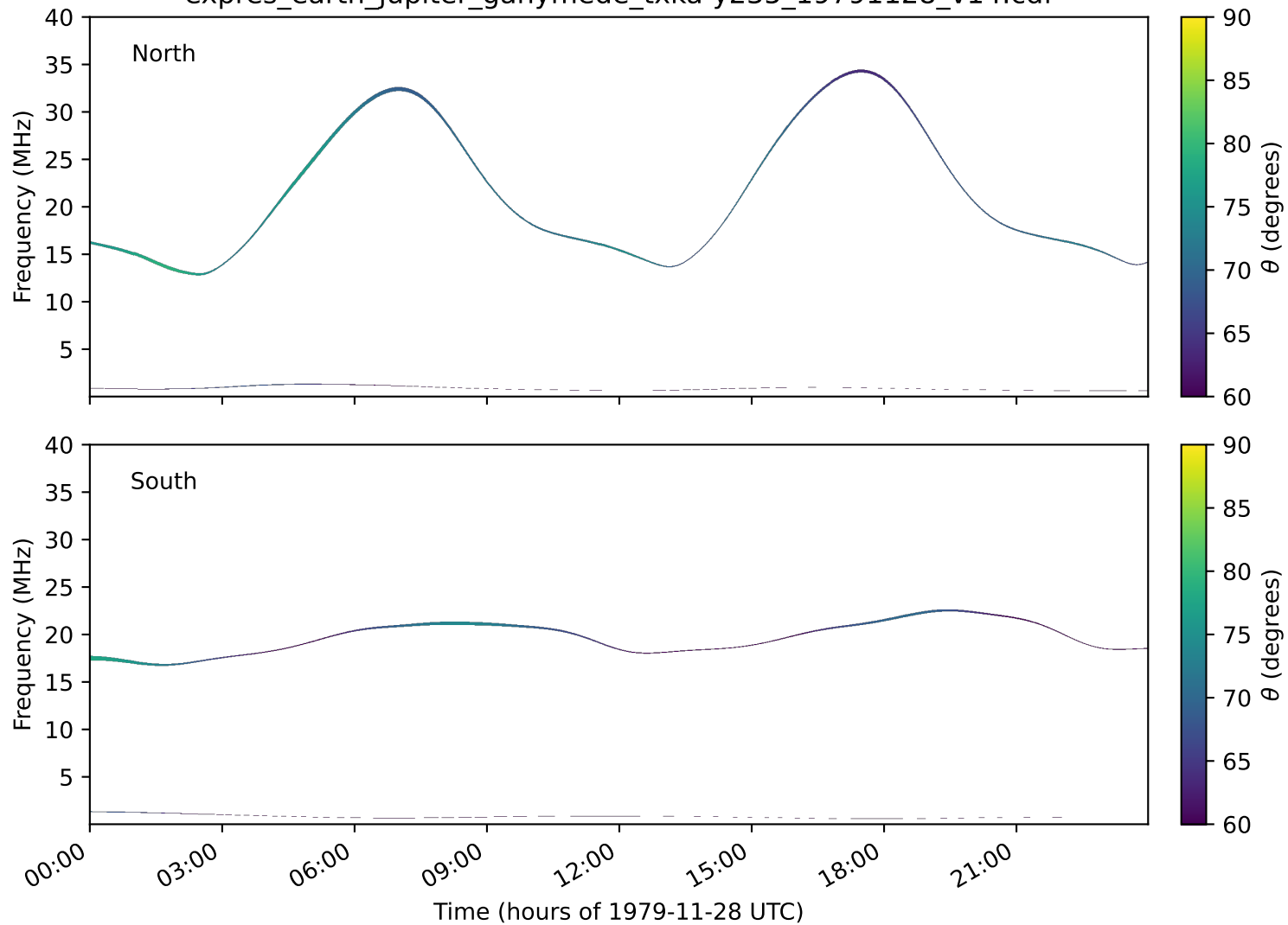
expres_earth_jupiter_ganymede_txka-y235_19791128_v14.cdf
