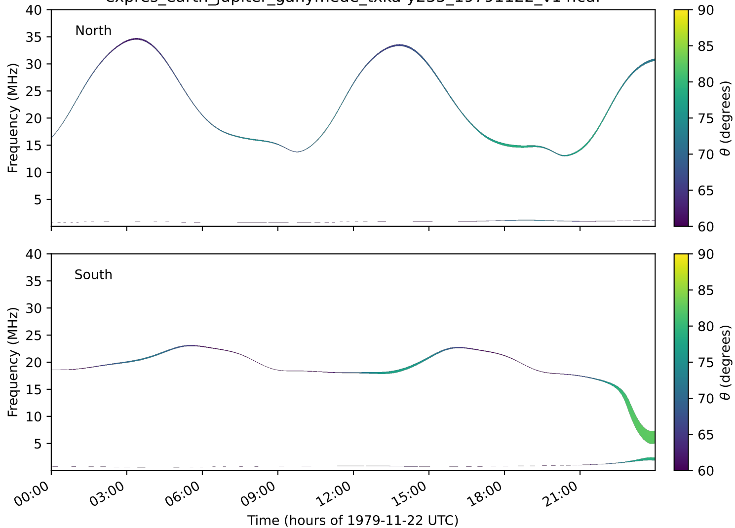
expres_earth_jupiter_ganymede_txka-y235_19791122_v14.cdf
