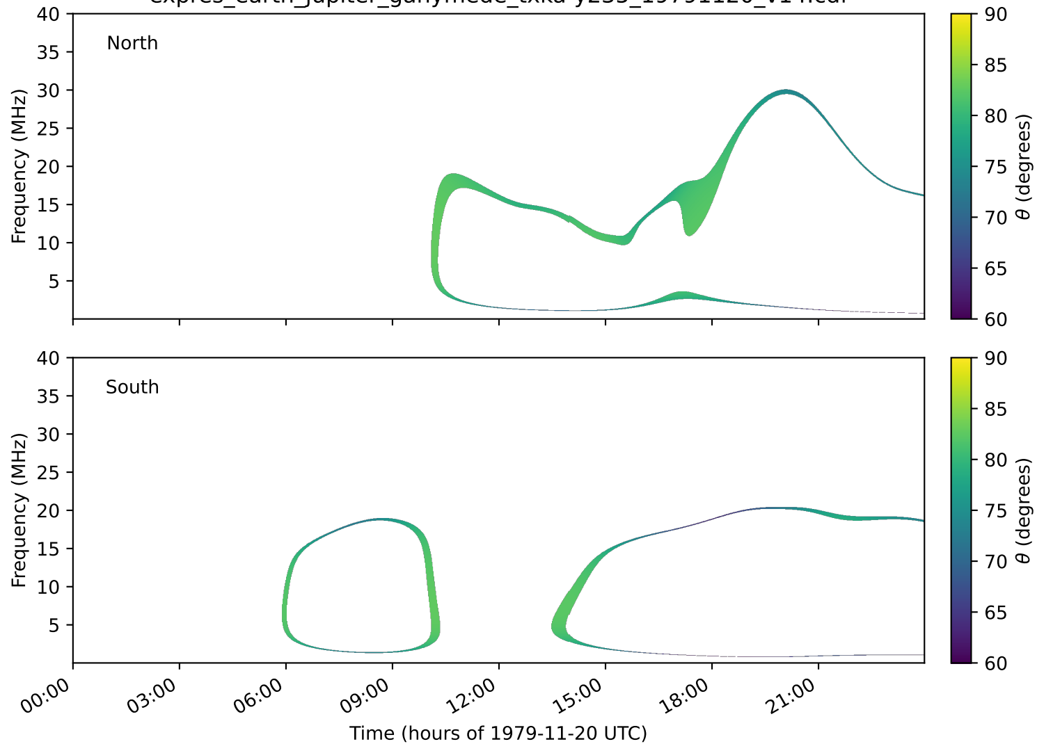
expres_earth_jupiter_ganymede_txka-y235_19791120_v14.cdf
