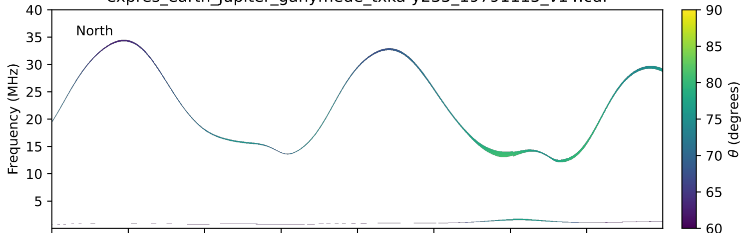
expres_earth_jupiter_ganymede_txka-y235_19791115_v14.cdf
