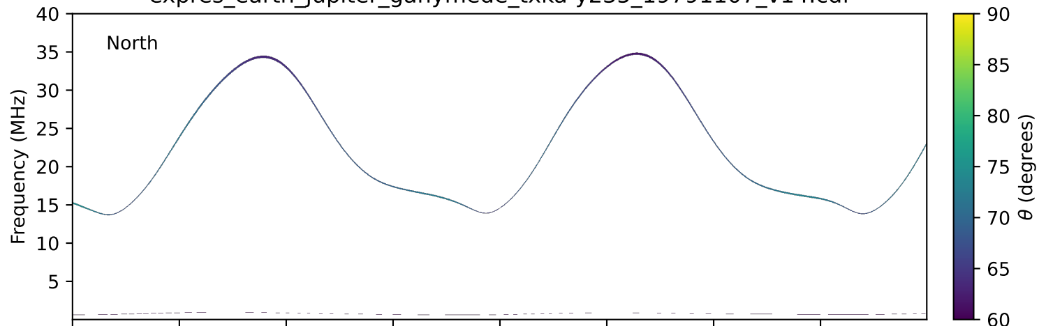
expres_earth_jupiter_ganymede_txka-y235_19791107_v14.cdf
