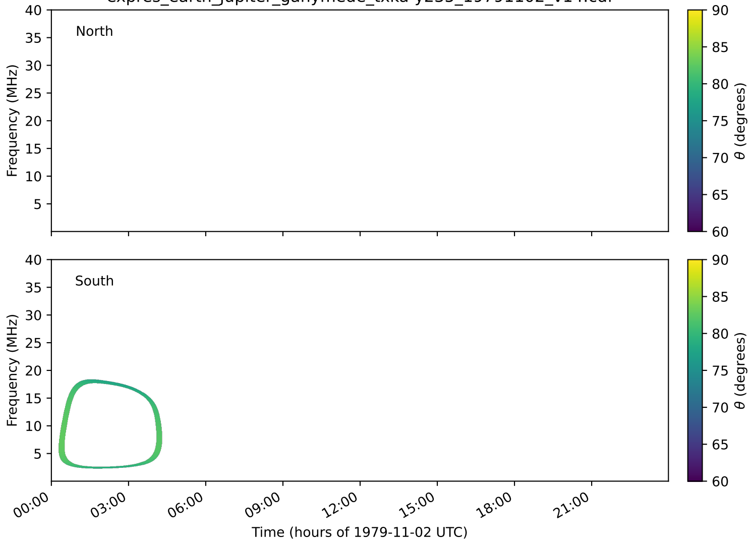
expres_earth_jupiter_ganymede_txka-y235_19791102_v14.cdf
