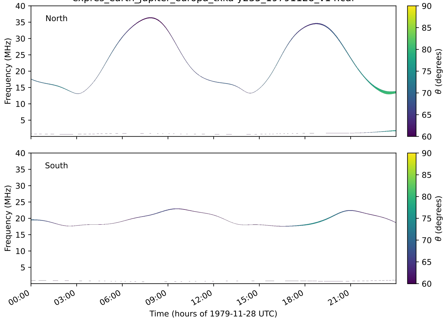
expres_earth_jupiter_europa_txka-y235_19791128_v14.cdf
