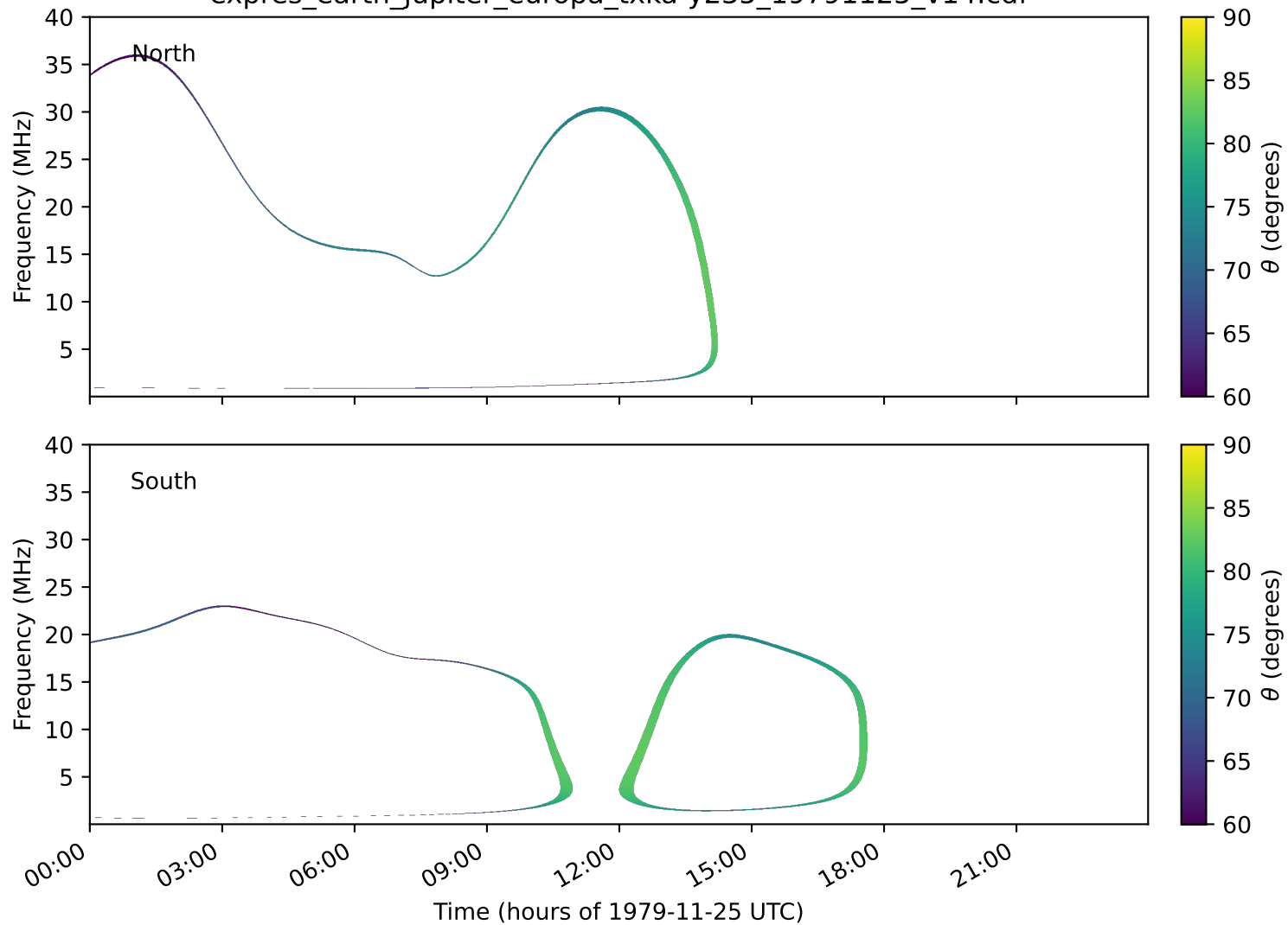
expres_earth_jupiter_europa_txka-y235_19791125_v14.cdf
