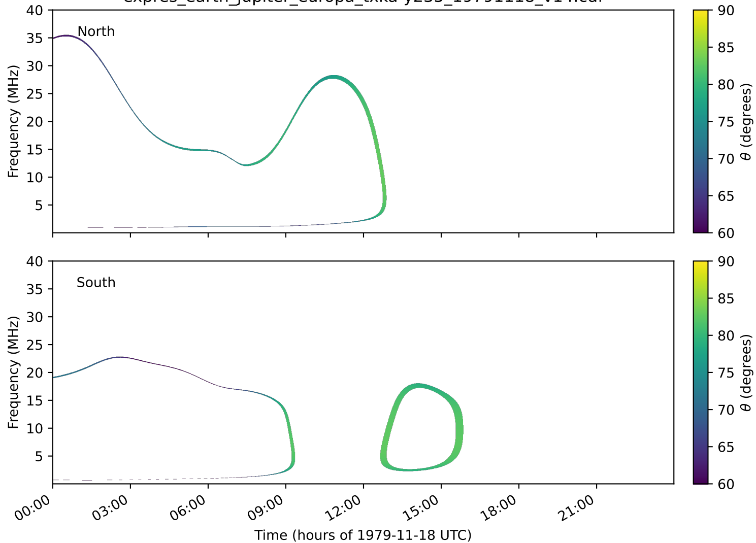
expres_earth_jupiter_europa_txka-y235_19791118_v14.cdf
