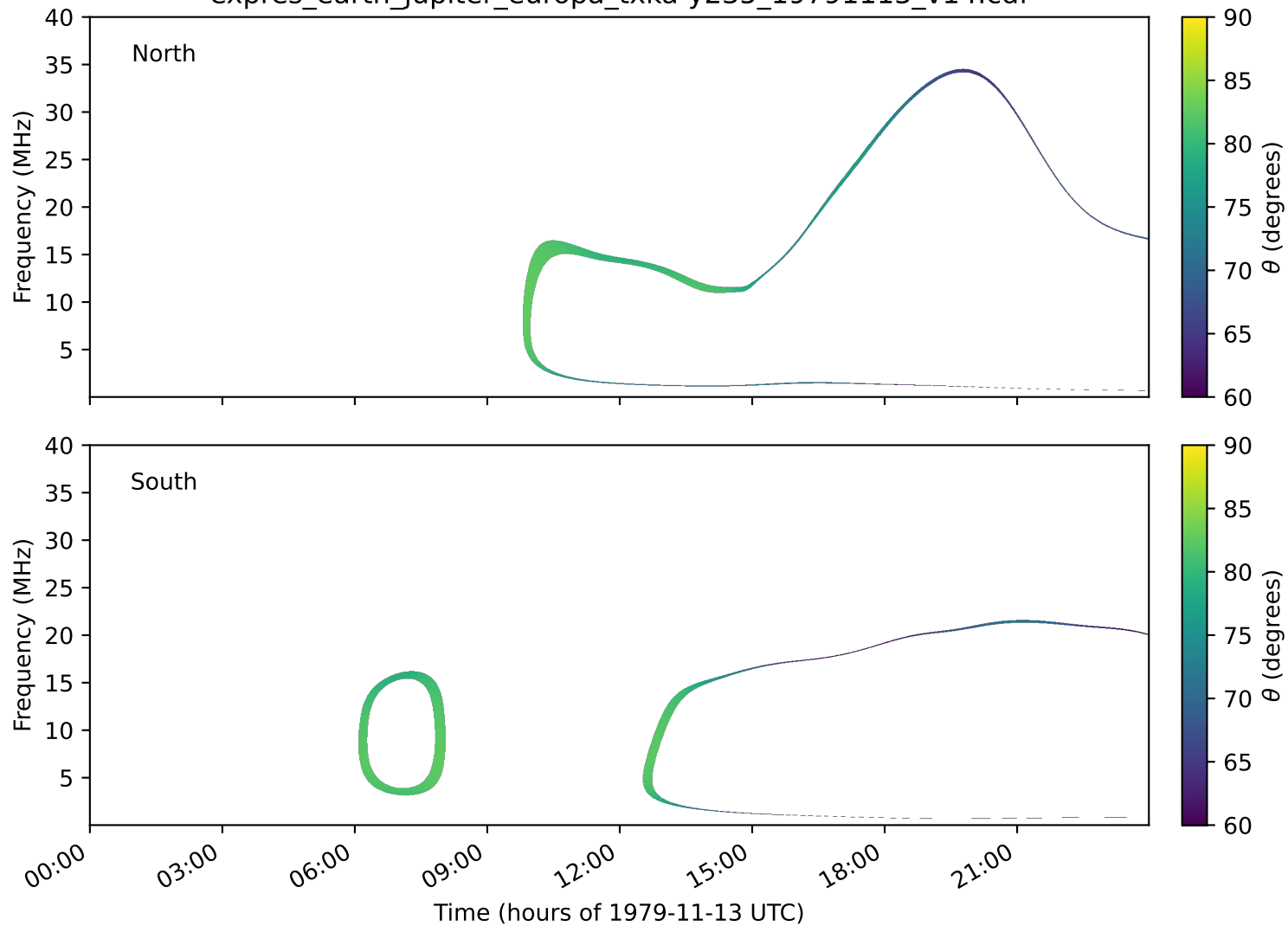
expres_earth_jupiter_europa_txka-y235_19791113_v14.cdf
