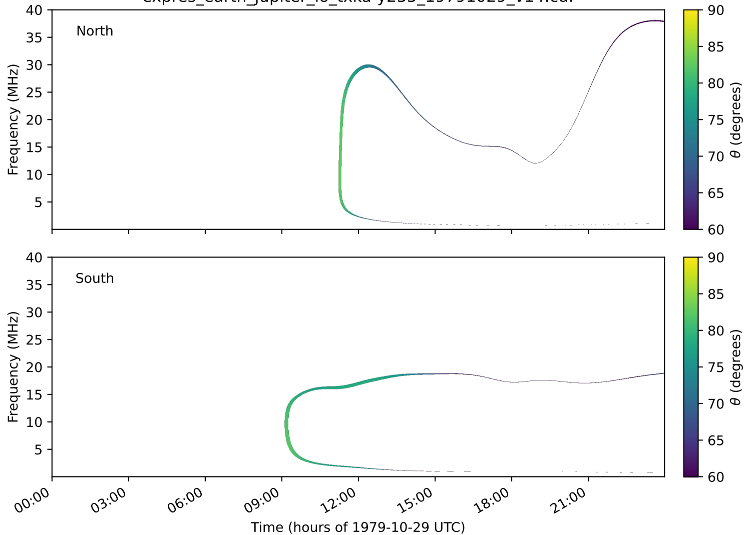
expres_earth_jupiter_io_txka-y235_19791029_v14.cdf
