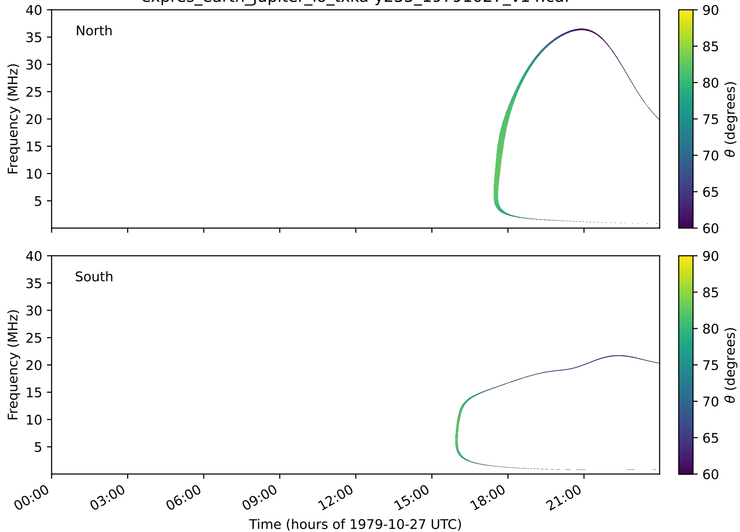
expres_earth_jupiter_io_txka-y235_19791027_v14.cdf
