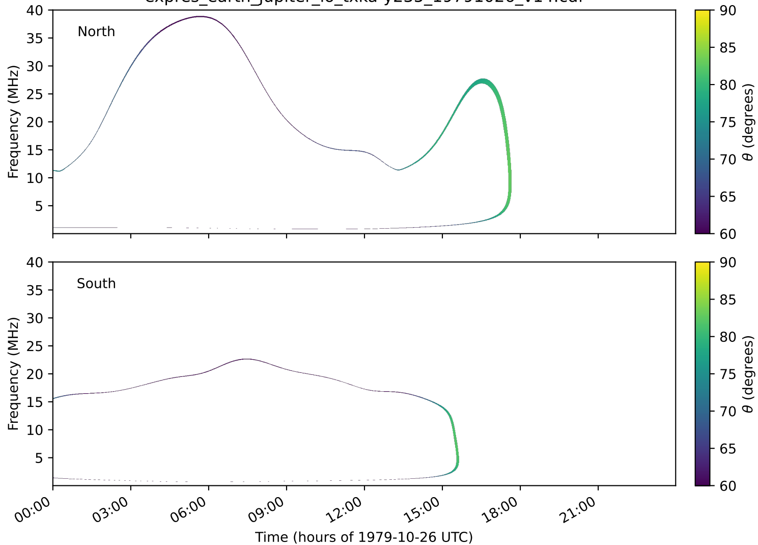
expres_earth_jupiter_io_txka-y235_19791026_v14.cdf
