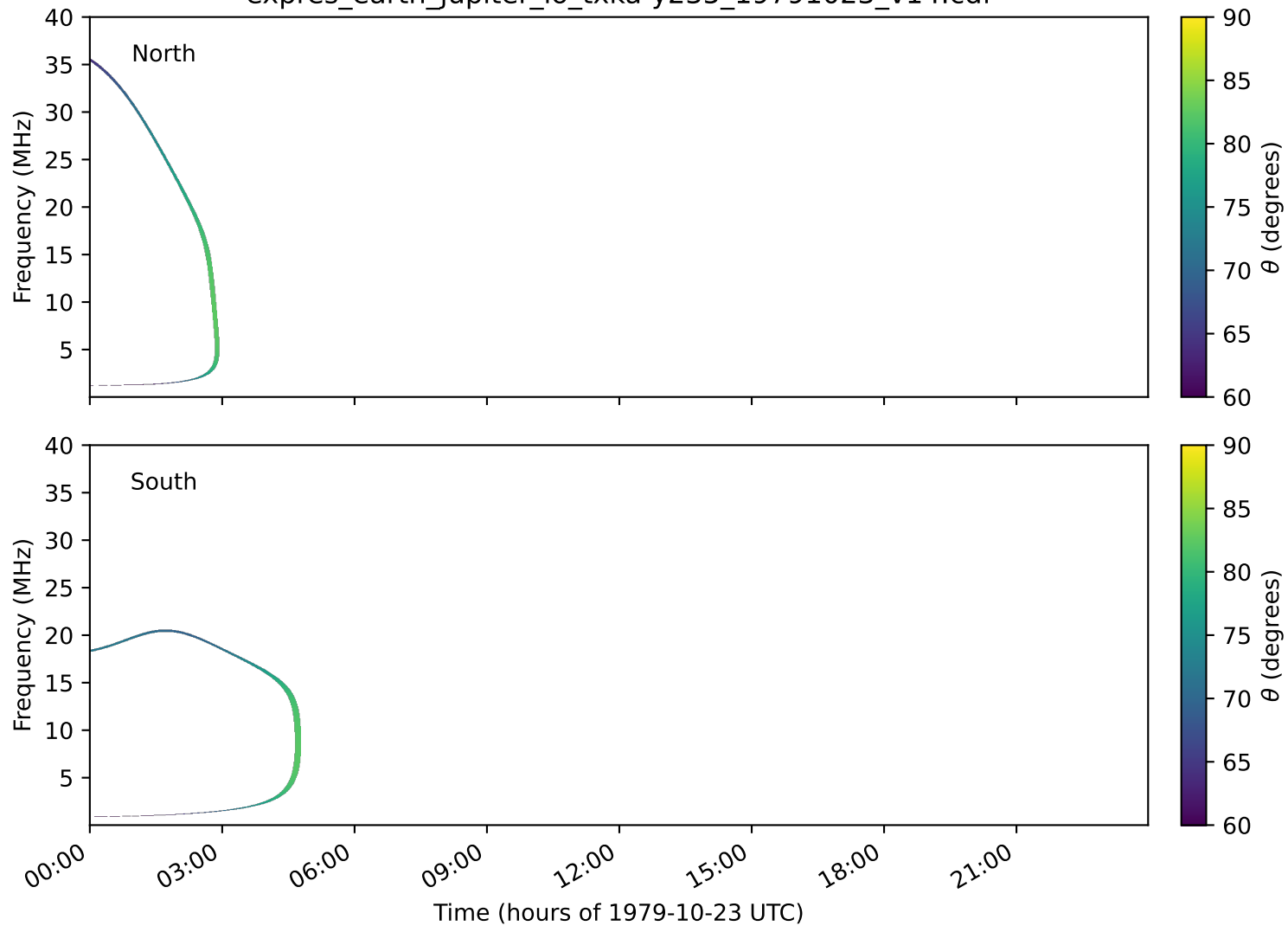
expres_earth_jupiter_io_txka-y235_19791023_v14.cdf
