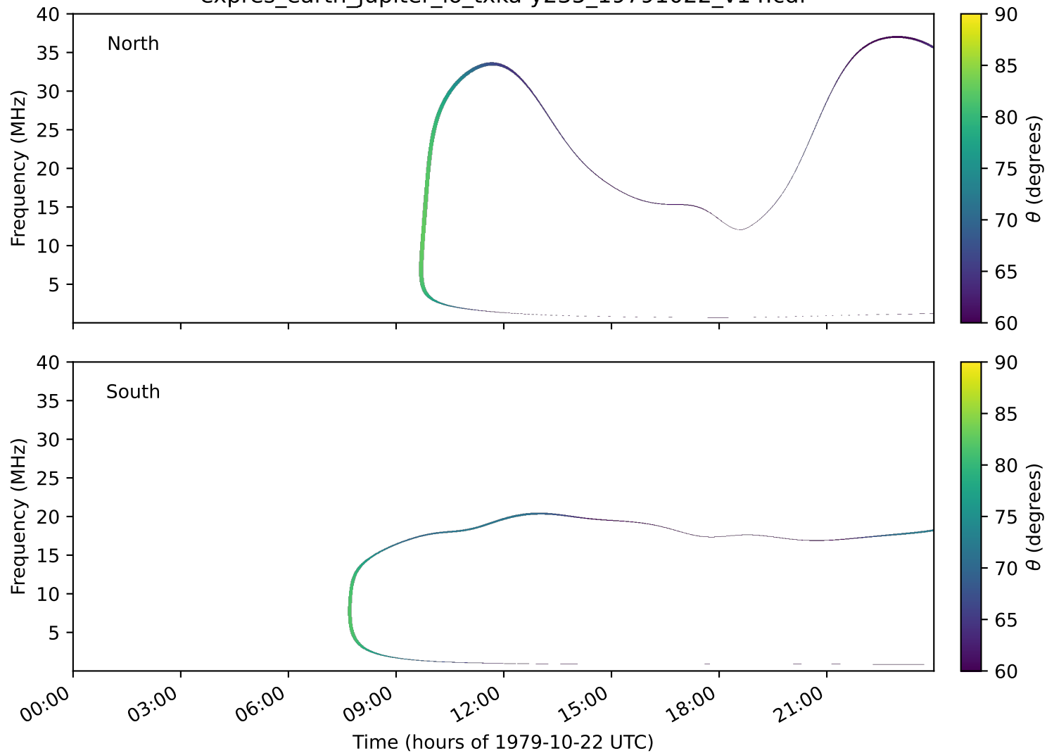
expres_earth_jupiter_io_txka-y235_19791022_v14.cdf
