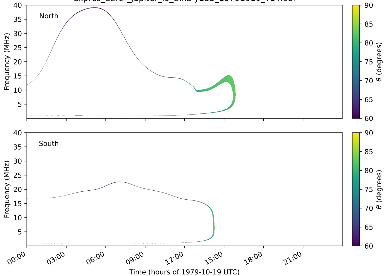
expres_earth_jupiter_io_txka-y235_19791019_v14.cdf
