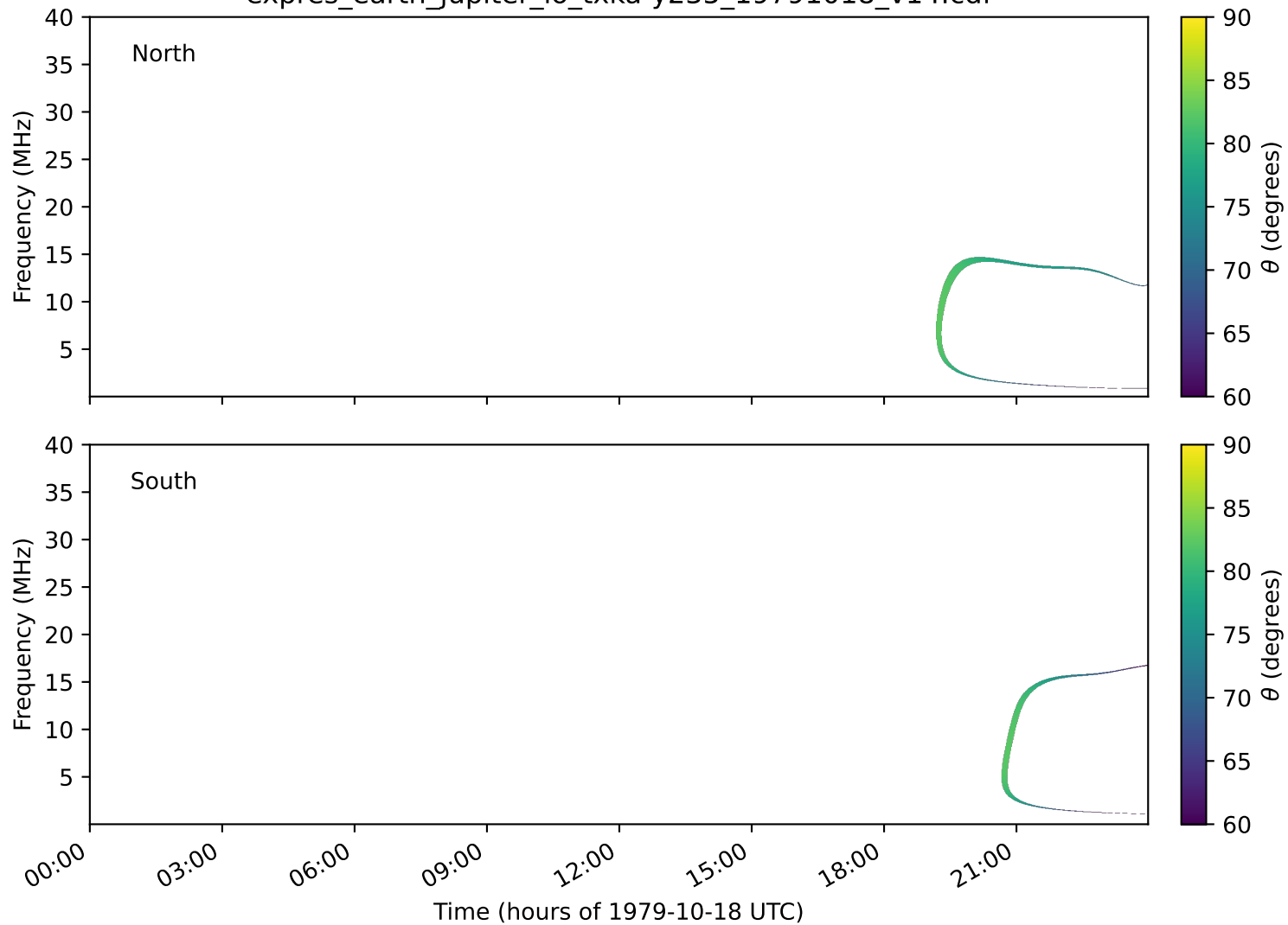
expres_earth_jupiter_io_txka-y235_19791018_v14.cdf
