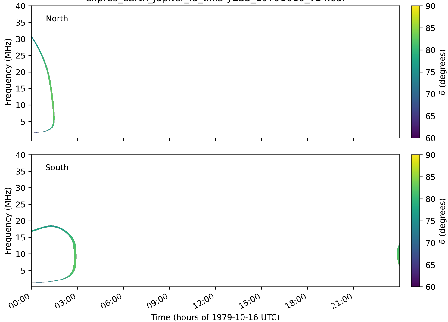
expres_earth_jupiter_io_txka-y235_19791016_v14.cdf
