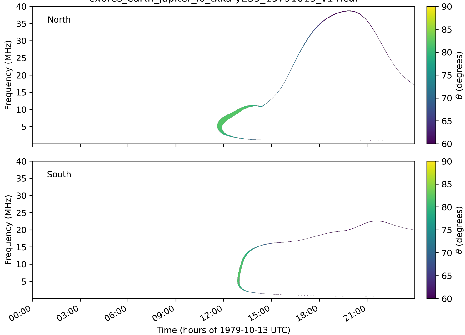
expres_earth_jupiter_io_txka-y235_19791013_v14.cdf
