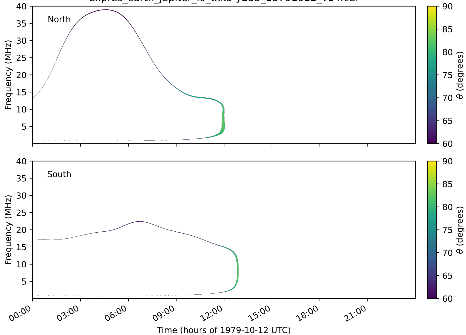
expres_earth_jupiter_io_txka-y235_19791012_v14.cdf
