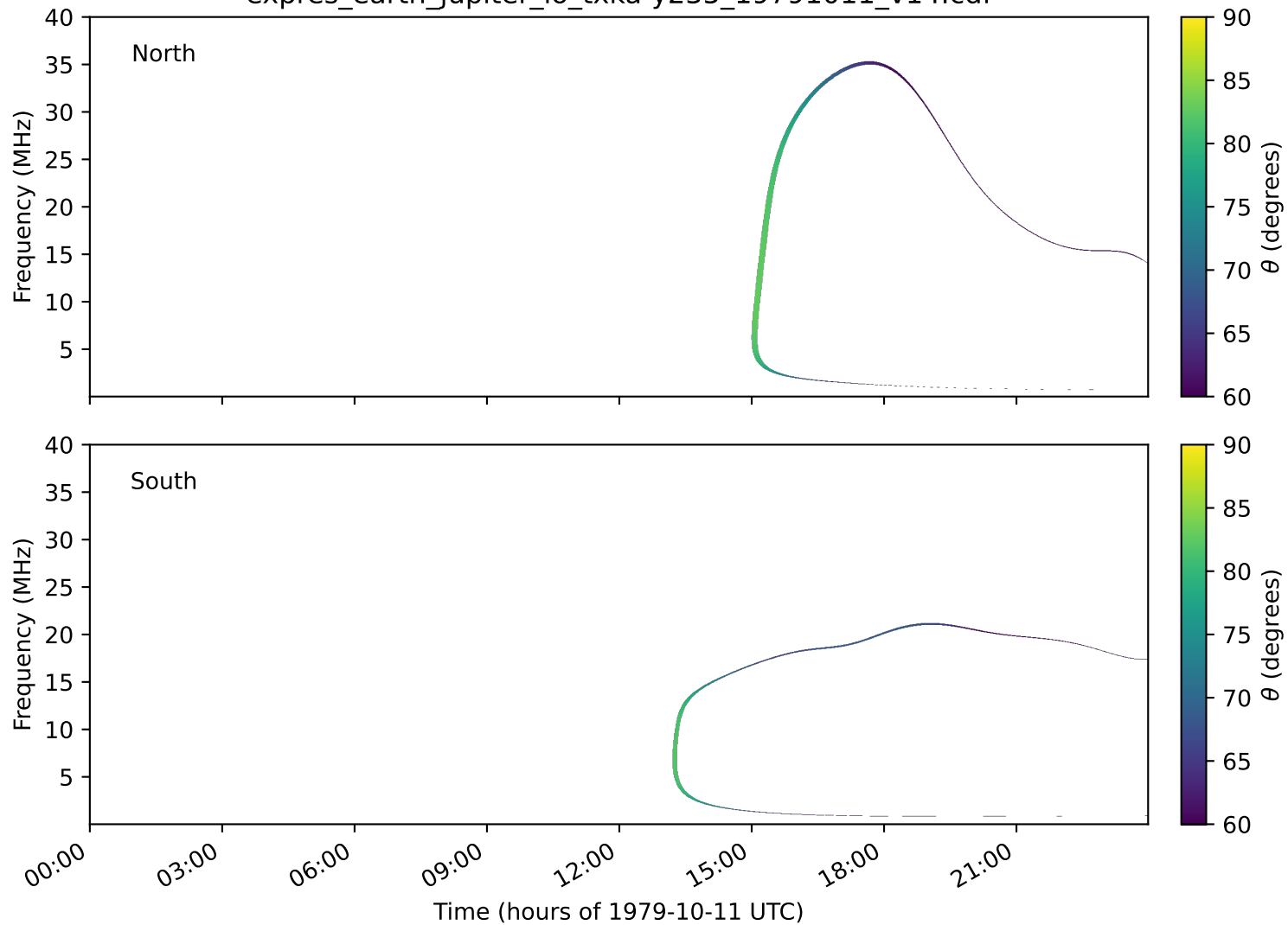
expres_earth_jupiter_io_txka-y235_19791011_v14.cdf
