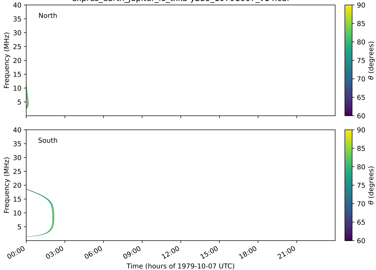
expres_earth_jupiter_io_txka-y235_19791007_v14.cdf
