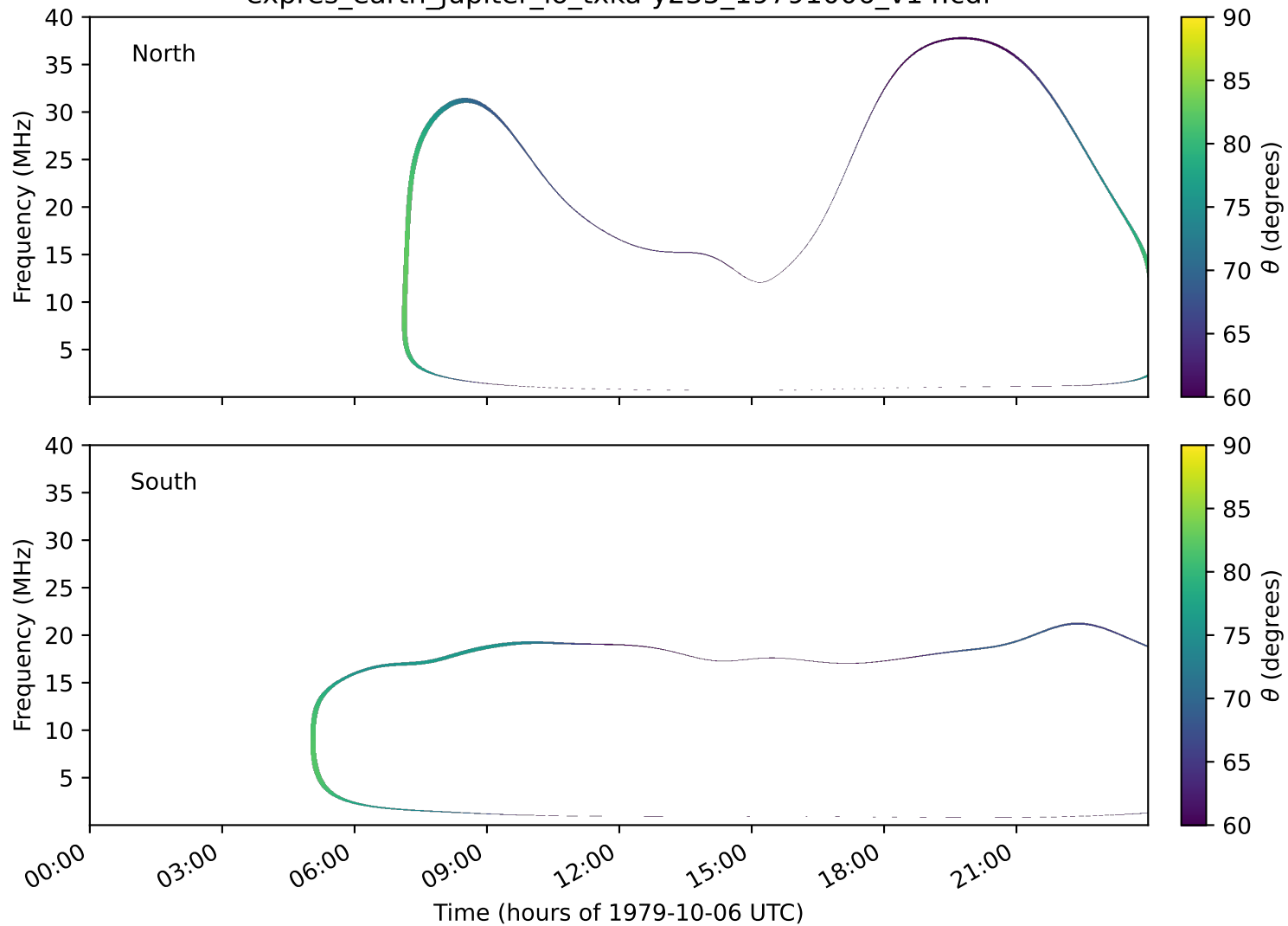
expres_earth_jupiter_io_txka-y235_19791006_v14.cdf
