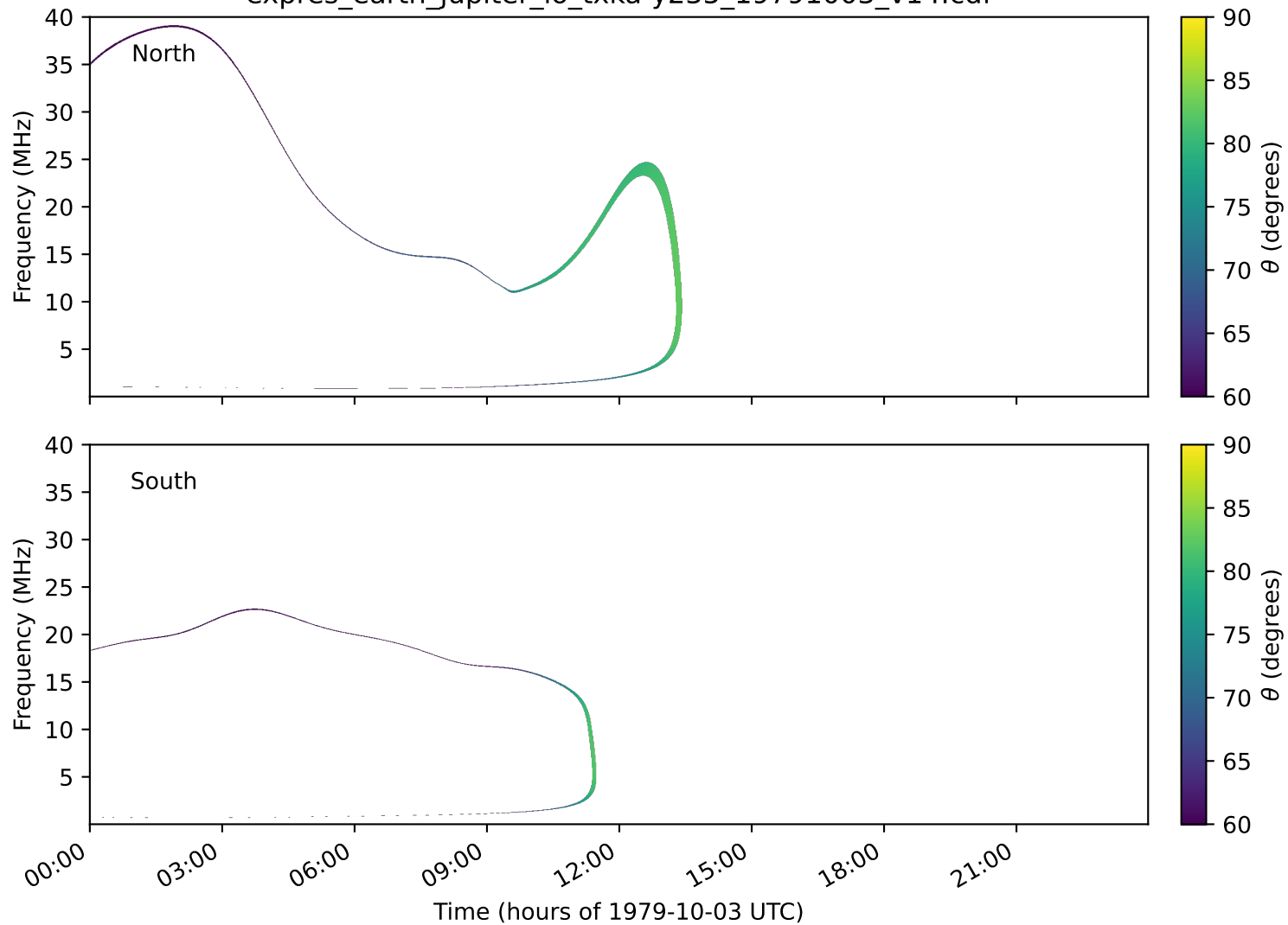
expres_earth_jupiter_io_txka-y235_19791003_v14.cdf
