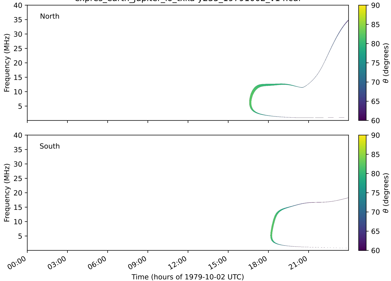
expres_earth_jupiter_io_txka-y235_19791002_v14.cdf
