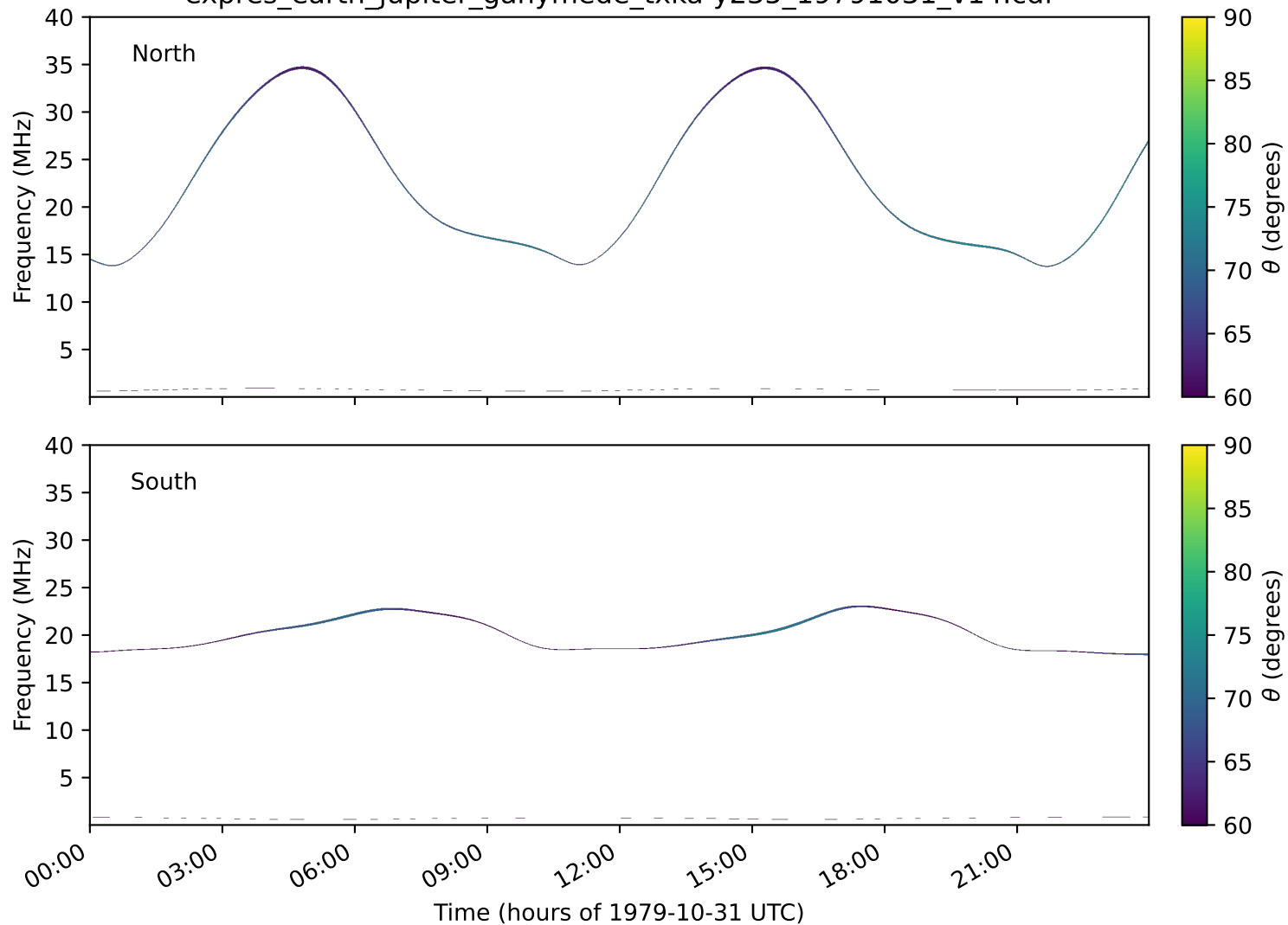
expres_earth_jupiter_ganymede_txka-y235_19791031_v14.cdf
