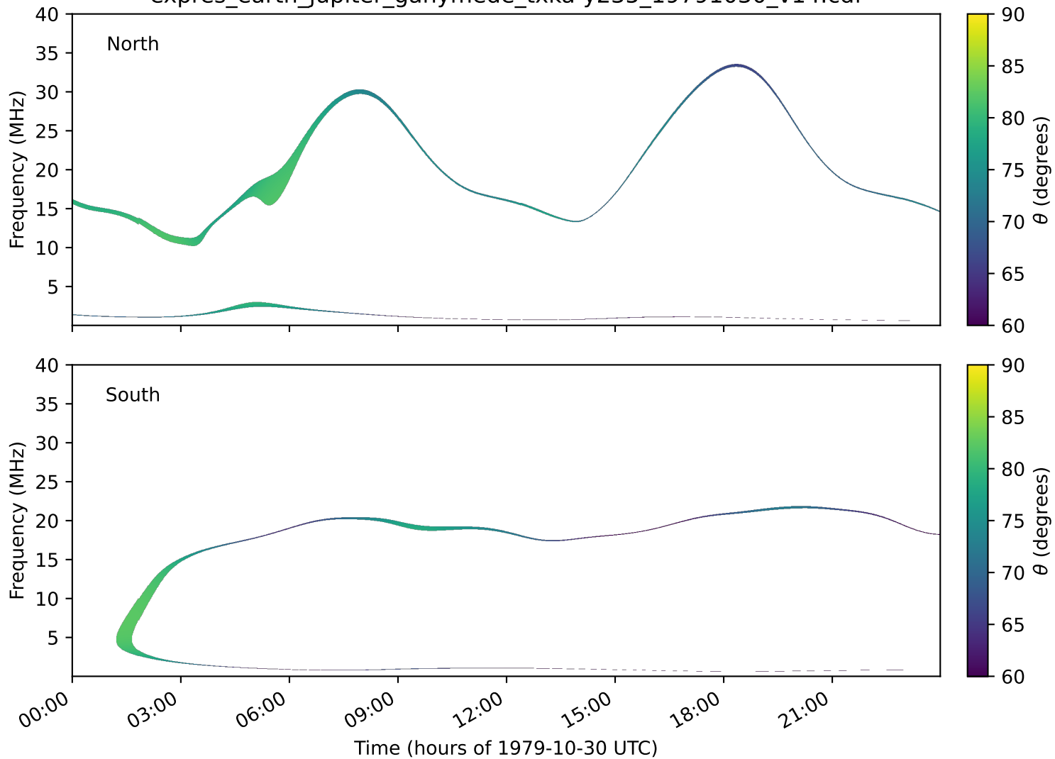
expres_earth_jupiter_ganymede_txka-y235_19791030_v14.cdf
